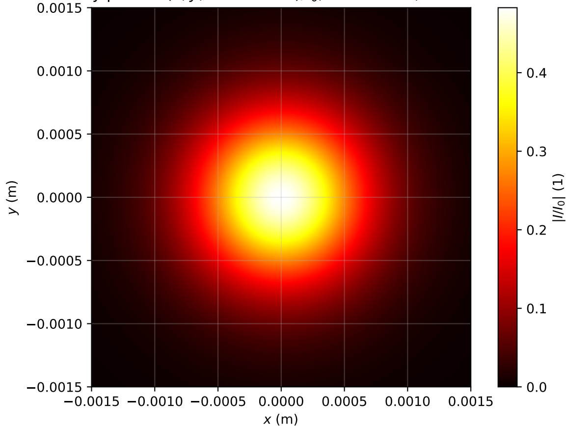
Intensity profile I(x, y, z = 3.981m)/I_0 , P_{in}=0.6P_{cr} , artificial time
